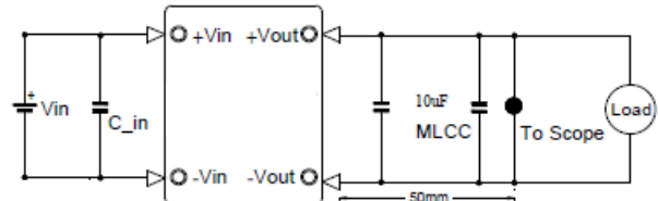
Figure 4. Measuring Output Ripple/Noise(20MHz bandwidth)
